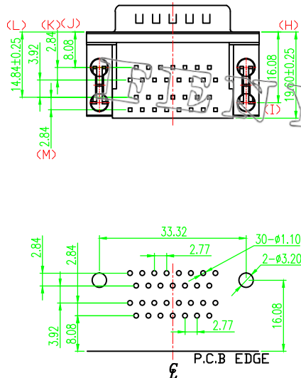
RECOMMENDED P.C.B LAYOUT INSPECTION DIMENSION:(A)~(M)
