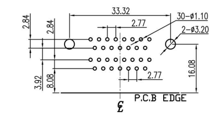
RECOMMENDED P.C.B LAYOUT INSPECTION DIMENSION:(A)~(M)
